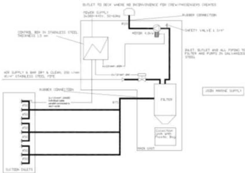
P&I Drawing, UCVC-40:
