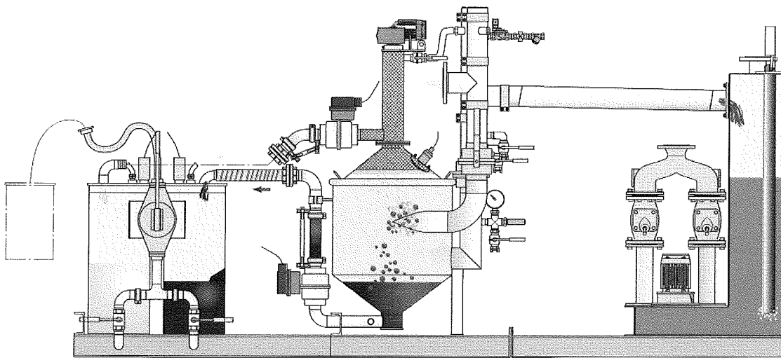
Grease / Sediment buffer tank and / or lift station (manual hand pump shown - high head electrical pumps also available)
